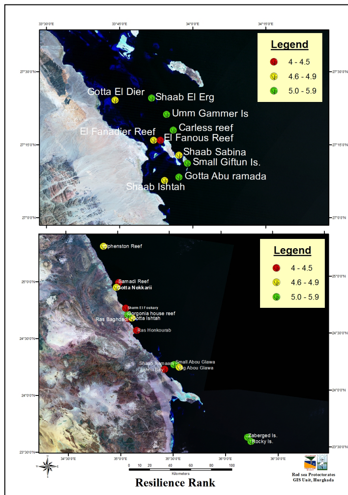
Figure (3) The distribution of northern and southern studied sites at the Egyptian Red Sea according to the resilience rank
