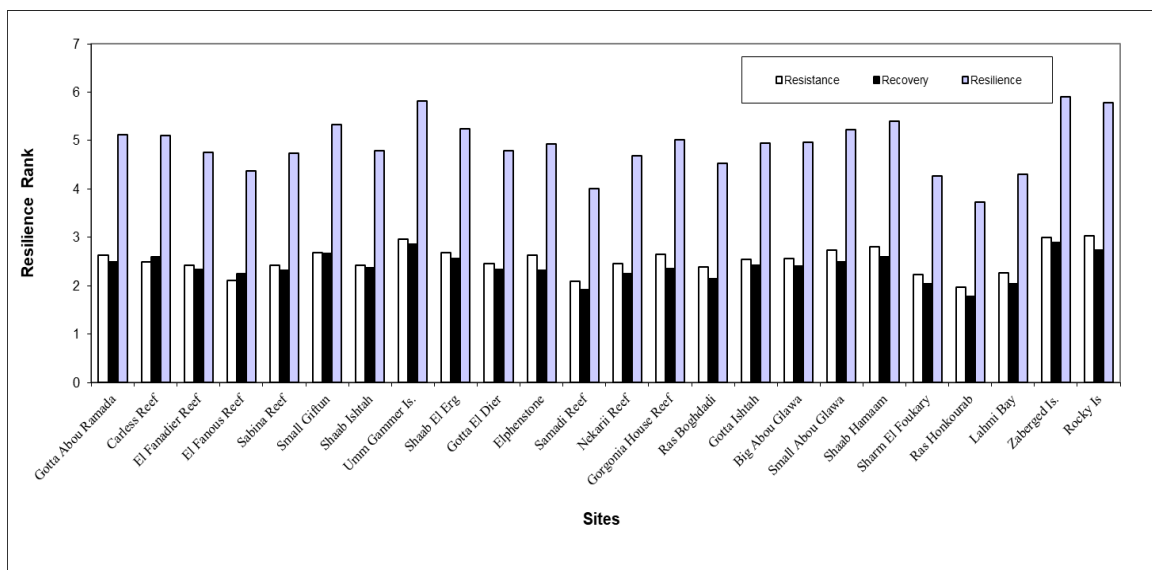
Figure (1) The rank of resistance, recovery and resilience at Egyptian Red Sea study sites
